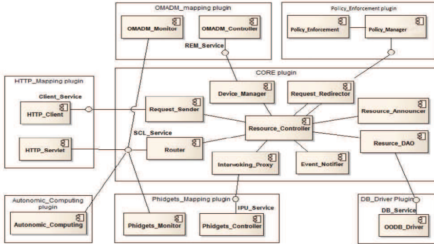
Figure 3. OM2M component diagram
