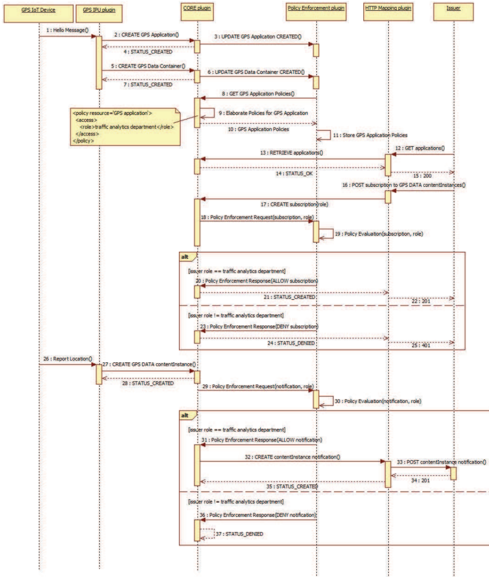
Figure 5. OM2M interactions with policy enforcement plugin
