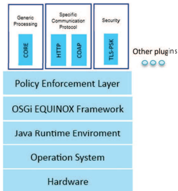
Figure 2. OM2M building layers
