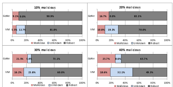
Fig. 7. Node classification - Topology 1
