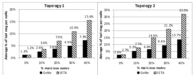
Fig. 6. Lost packets
